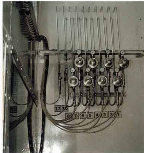
FLUID OUTLET PAINT REGULATOR 塗料取出口穩壓器 (270-050)
