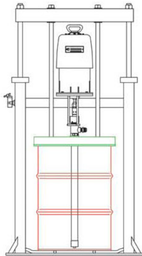
55 Gallon two post drum cover 55加侖雙昇降氣缸式
