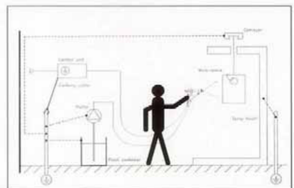
Installation diagram for electrostatic system
