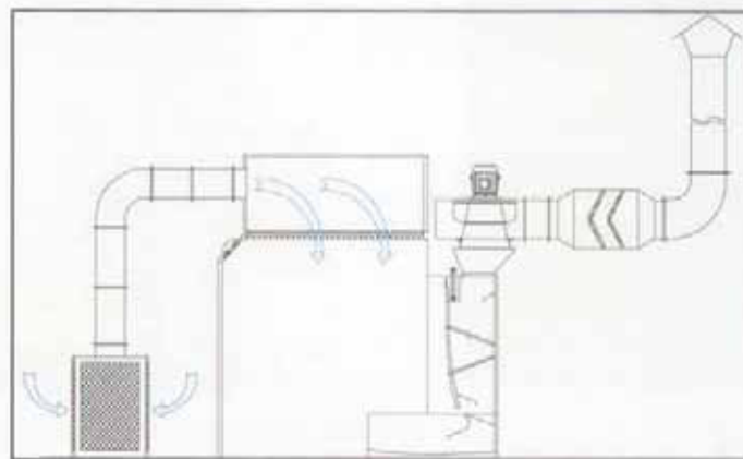
Air supplier, exhaust air system and Charcoal filter system
